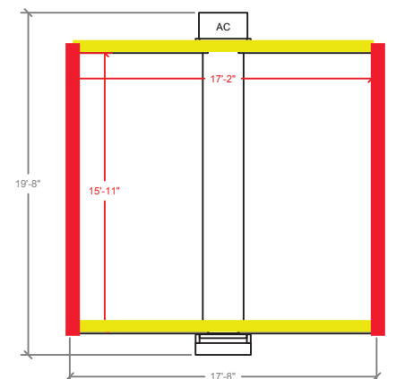
SINGLE UNIT
